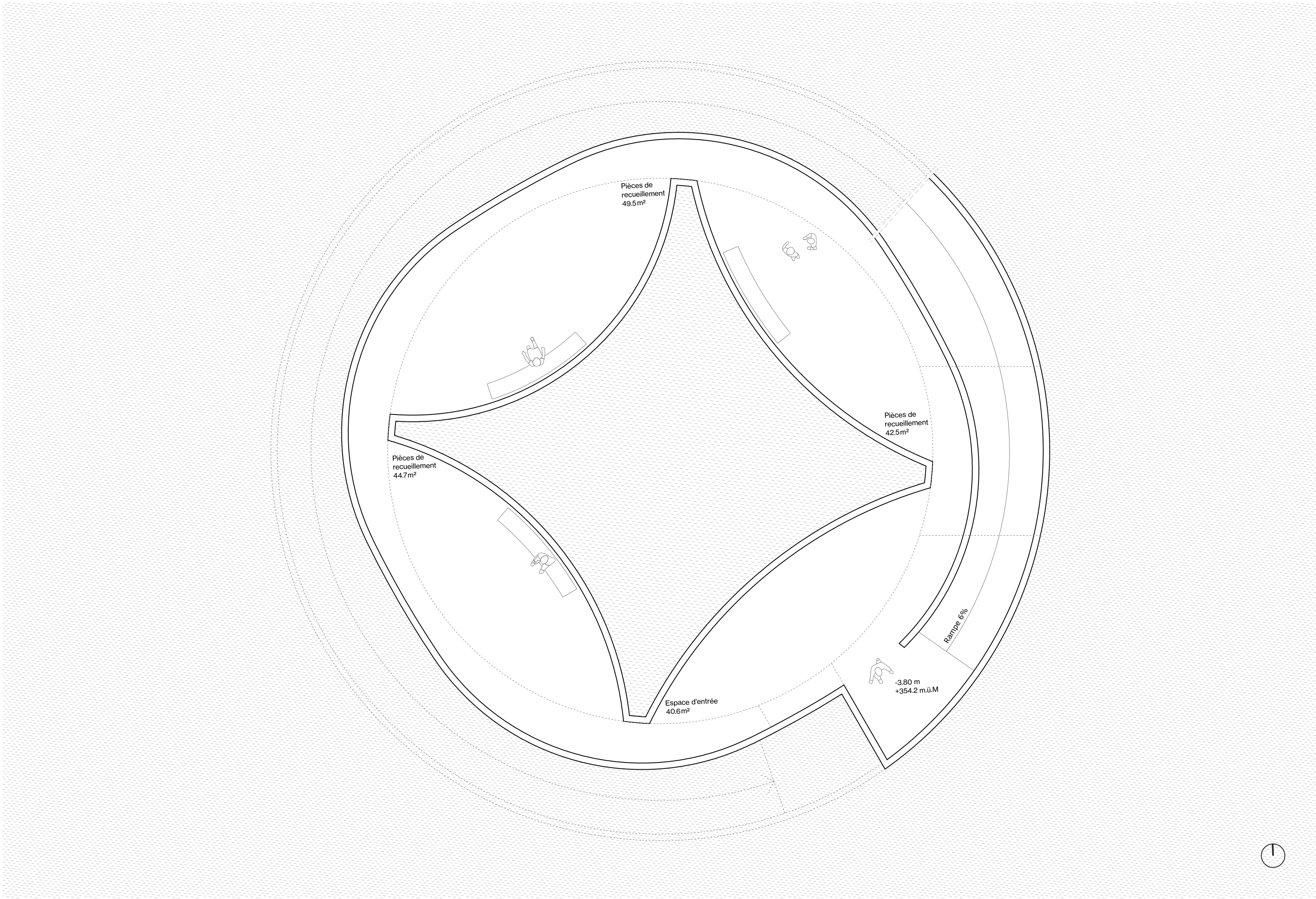
Plan R-1 1/100
